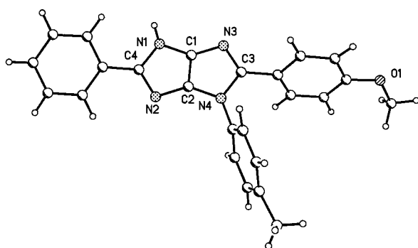
Figure 3. Representation of the molecular structure of 11b ; the numbering corresponds to that used for the X-ray analysis; selected distances [Å] and angles [°]: C1–C2 1.361(2), C2–N2 1.369(2), N2–C4 1.369(2), C4–N1 1.386(2), N1–C1 1.376(2), C1–N3 1.374(2), N3–C3 1.346(2), C3–N4 1.398(2), N4–C2 1.389(2); C4–N2–C2 102.2(1), C4–N1–C1 105.2(1), C1–N3–C3 102.9(1), C3–N4–C2 105.6(1)
