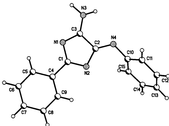
Figure 2. Perspective drawing of 3f ; the numbering corresponds to that used for the X-ray analysis; selected distances [Å] and angles [°]: C3–N1 1.329(2), N1–C1 1.408(2), C1–N2 1.329(2), N2–C2 1.399(2), C2–C3 1.511(2), C3–N3 1.319(2); C3–N1–C1 102.7 (1), C1–N2–C2 103.3(1), N2–C2–N4 131.1(1), N1–C3–N3 127.3(1)
