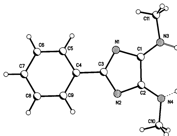
Figure 1. X-ray structure of 4c ; the numbering corresponds to that used for the X-ray analysis; selected distances [Å] and angles [°]: C1–N1 1.378(2), C3–N1 1.351(2), N2–C3 1.375(2), N2–C2 1.358(2), C1–C2 1.508(2), C1–N3 1.297(2), C2–N4 1.308(2); N1–C1–N3 127.4(1), N2–C2–N4 126.7(1), N1–C3–N2 118.7(1), N2–C2–C1 108.3(1), N1–C1–C2 107.3(1)
